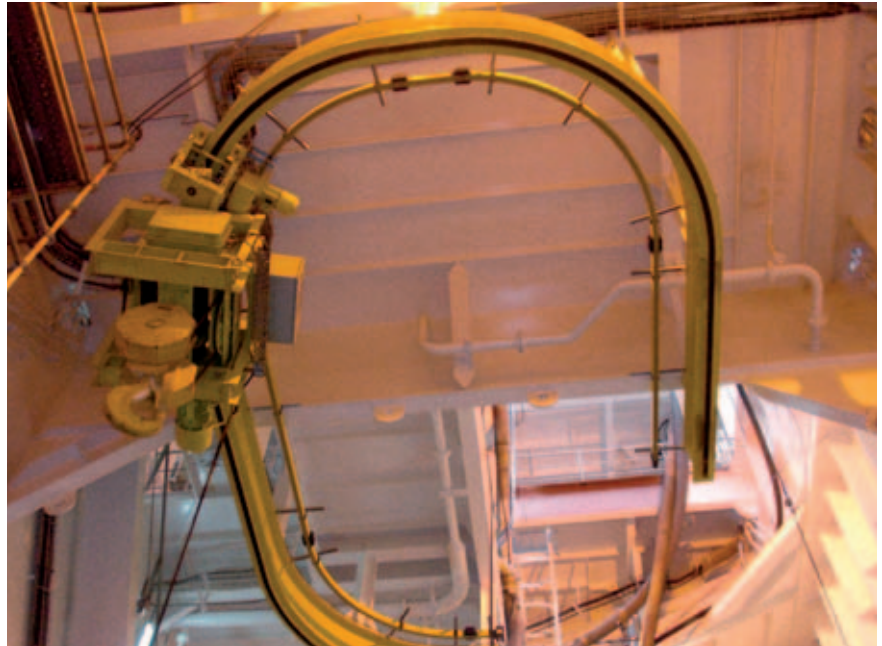
SWL 25.0t Radius 1800mm Class BV
