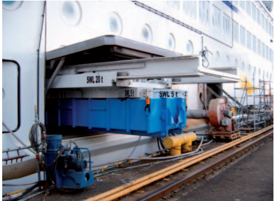
Garbage Container Crane SWL 20t Class DNV
